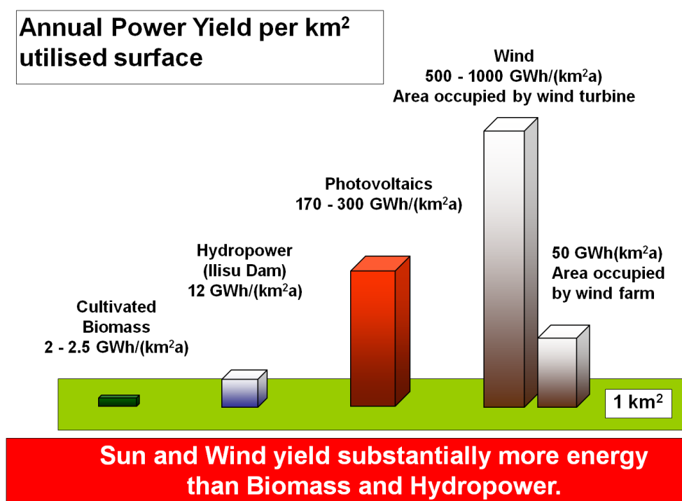
Figure 1: Annual power yield per km 2 utilized surface
